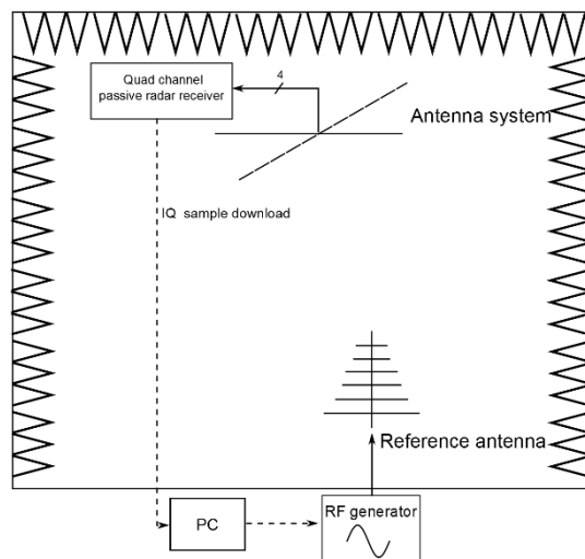
Fig. 4. Calibration measurement setup
