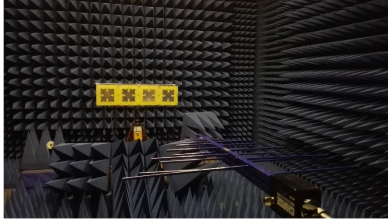
Fig. 5. Calibration measurement taken in the anechoic chamber
